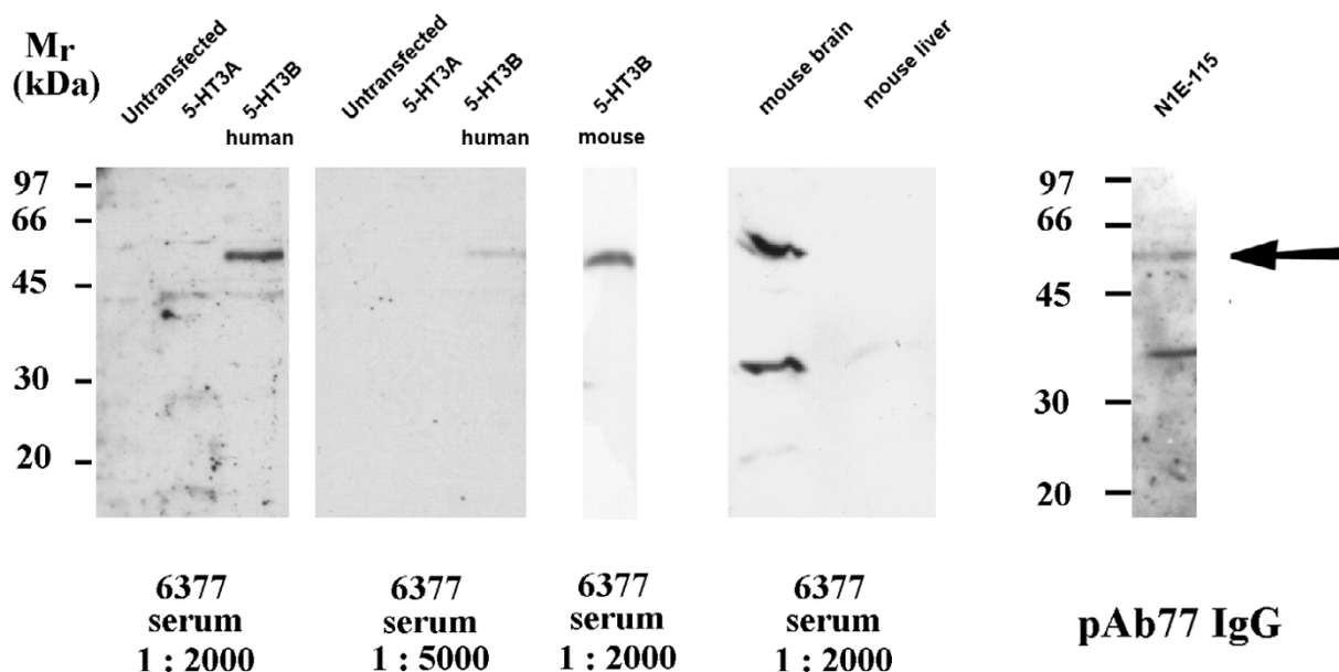
Figure 1 Western blots of lysates from untransfected HEK293 cells and HEK293 cells expressing mouse 5-HT 3A or 5-HT 3B receptor subunits, or human 5-HT 3B receptor subunits. Blotted membranes were hybridised with dilutions of 6377 serum or purified pAb77 IgG fraction as the primary antibody. Data are typical of three or more independent experiments. The arrow indicates the position of 5-HT 3B receptor subunits. Western blots using lysates from mouse tissues and NIE-115 cells are shown on the right hand side.
