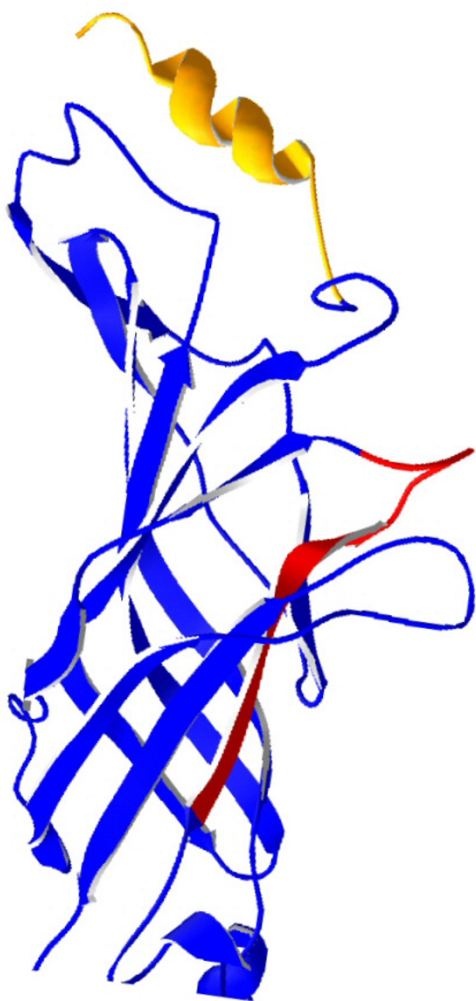
Figure 3 Model of the 5-HT 3B receptor subunit extracellular domain. based on the structure of the nicotinic acetylcholine receptor, showing the location of peptides corresponding to those used as immunogens for pAb77 (yellow) and AP86/3 (red).
