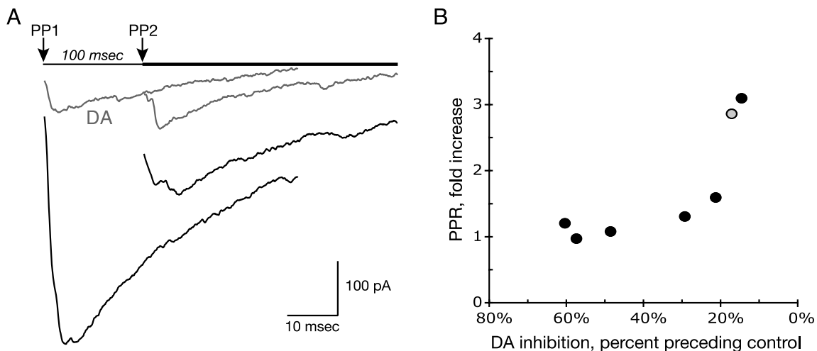
Figure 4 Paired-pulse facilitation. A. Paired pulses (PPI and PP2) were delivered at a 100 msec interval in the absence (saline, black traces) and the presence of DA, 1 μM (gray traces). In this experiment, DA produced a dramatic inhibition to 17% of control, which was accompanied by about a 3-fold increase in the paired-pulse ratio (PPR), from 0.47 to 1.34. Traces shown are the averages of 5 traces. B. Plotting PPR vs. DA inhibition (expressed as the percent of the preceding control IPSC) for all paired-pulse experiments (n = 8), showed that PPR increased with DA modulation, indicative of presynaptic action. The gray-filled circle, corresponds to the experiment shown in panel A.
