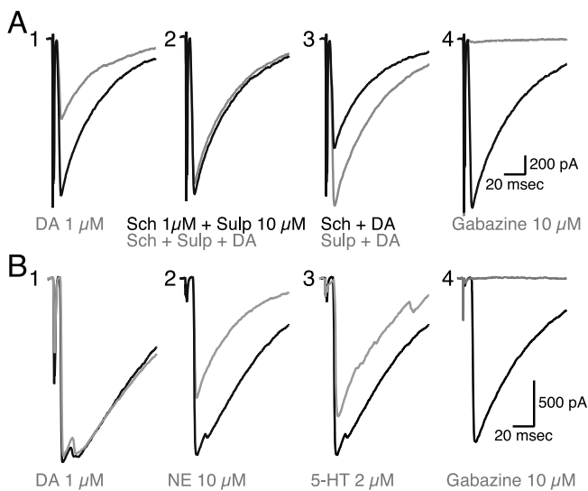
Figure 3 Neurotransmitter modulation of autaptic response. A. Here, a high-chloride intracellular solution was used so that autaptic responses were inward and larger. (A1) DA (gray trace) inhibited the autaptic response, here to 52% of control. (A2) Application of the D1 antagonist SCH23390 (SCH) together with Sulpiride (Sulp) had no impact on the response (black trace), but blocked DA action (gray trace). (A3) In this experiment, the DA inhibition was D2-mediated, as Sulpiride blocked DA action completely (gray trace), while SCH23390 had only a modest effect. (A4) At the end of the experiment, gabazine (gray trace) completely blocked the autaptic response. B. In another cell, (B1) the autaptic connection did not show DA modulation. However, (B2) Norepinephrine (NE; 68% inhibition) and (B3) Serotonin (5-HT; 78% inhibition) inhibited the autaptic response, arguing that DA does not act through other monoamine receptors. (B4) At the end of the experiment, the autaptic response was completely blocked by Gabazine.
