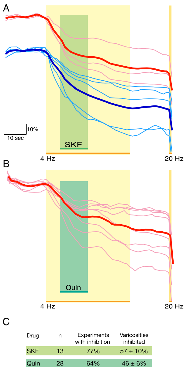
Figure 5 Imaging presynaptic modulation by FMI-43 destaining. Synaptic vesicles were loaded (stained) with FMI-43 by field stimulation, and then imaged every 1.25 sec. After a control period (15 images), showing that there was limited bleaching, field stimulation was applied at 4 Hz; destaining was monitored at 8 varicosities (thin traces). A. During this stimulation, the D1 agonist SKF38393 (SKF, 10 μM) was perfused (10 images). For 5 varicosities (blue traces), there was no inflection in the destaining curve, while in the others (red traces), the destaining was arrested, creating an inflection. The two thick traces are averages of the sets of effect and no-effect traces. The effect traces were offset upwards for the sake of the illustration. Once the SKF38393 was washed off, and the stimulation continued, destaining continued or resumed. After an interval of no stimulation, the remaining FMI-43 was unloaded with a 20 Hz tetanus. A total of 70 images were acquired. B. In another culture, the D2 agonist Quinpirole (Quin, 1 μM) was applied. In this experiment all 8 varicosities showed inhibition (red traces). D2 effects typically had a greater latency; note that the plateau started roughly when the drug was washed off (presumably coincidental). C. Overall, the majority of experiments showed either D1 or D2 inhibition, and in those experiments about half of varicosities showed inhibition (expressed as mean ± s.e.m.). Facilitation, as would be reflected in an increase in the destaining rate, was not seen. In each of the 13 D1 agonist experiments, a minimum of 2 varicosities showed inhibition; in the 18 D2 agonist experiments, 3 experiments had only one varicosity that showed inhibition. In one D1 agonist experiment and in one D2 agonist experiment every varicosity showed inhibition.
