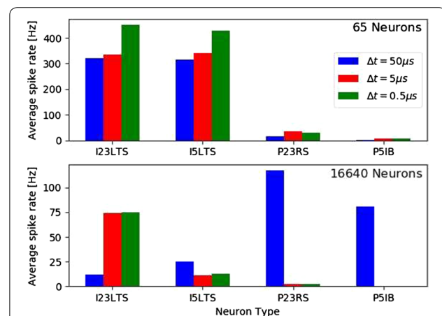
Fig. 1 Average spiking rates for excitatory pyramidal neurons in layer 2/3 (P23RS) and layer 5 (P5IB) and inhibitory neurons in layer 2/3 (I23LTS) and layer 5 (I5LTS) for the three time step sizes used in this study
